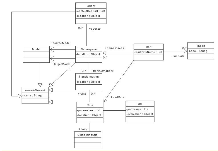
Figure 1 Abstract Syntax
